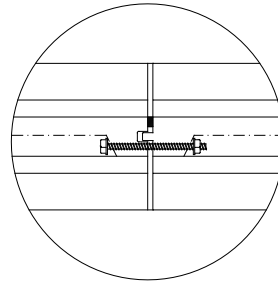
JOINT AND SEALANT DETAIL
