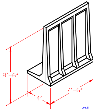
8'-6" L-Panel
