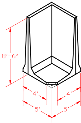
8'-6" Corner Panel
